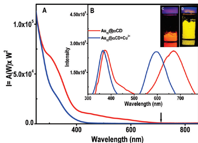
Figure 6. (A) UV-vis spectra and (B) PL spectra of the Au 15 @ \alpha CD cluster before and after the addition of Cu 2+ . Insets show photographs of the cluster powder under UV light before the addition of Cu 2+ (inset C) and after the addition of Cu 2+ (inset D).
